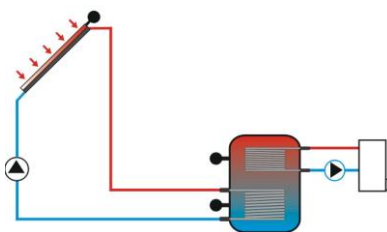
Heat tank to constant temperature
